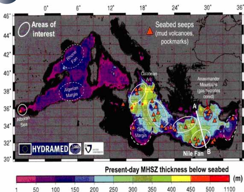
Figure 2. Modelled methane hydrate stability zone for present-day conditions, with areas of interest for hydrate occurrence; orange triangles indicate the general locations of known seabed seeps (various sources).
